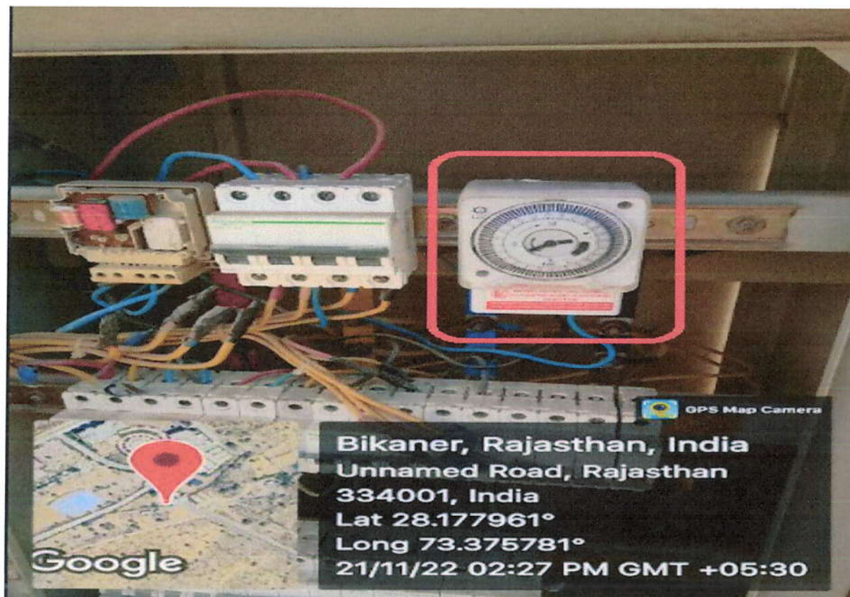
Instrument with Timer for Street Lights Control
